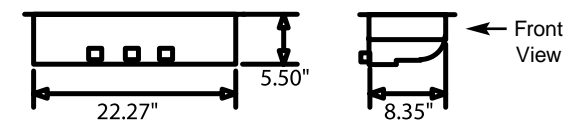
#52400 460 Ford 3 pick-up Dry Sump Pan
