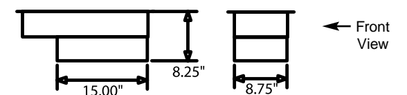
#55365 351C SB Ford (Cleveland) Wet Sump Pan (original design-Pantera) #55432 460 Ford Wet Sump Pan (Pantera)
