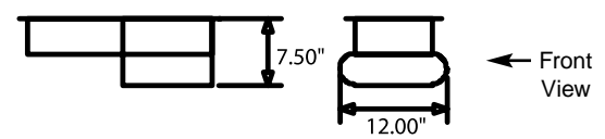
#55350 302 SB Ford 7.5: Wet Sump Pan (original GT 350 "R" model) #55351 351 SBW Ford 7.5: Wet Sump Pan (original GT 350 "R" model)
