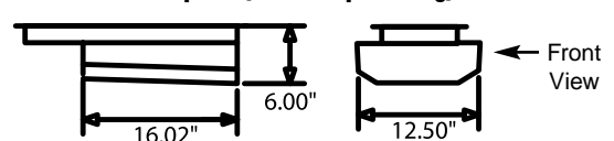
#55410 Ford FE Wet Sump Pan (original 427 Cobra) #55412 Ford FE Wet Sump Pan (front sump Mustang)
