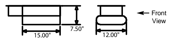
#55355 302 SB Ford Wet Sump Pan (original 289 Cobra) #55356 351 SBW Ford Wet Sump Pan (original 289 Cobra)
